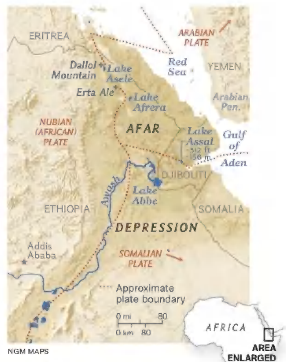
Located at the intersection of three geologic plates, the Afar depression is caught in a tectonic tug-of-war that's splitting off part of the continent.
